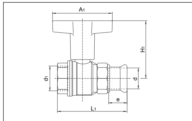
Codice 107 71 52 – 56 (G 1/2 x Ø 15 – G 1 1/4 x Ø 35),
