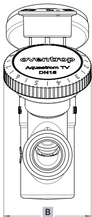
Fig. 3: Frontal dimensions
