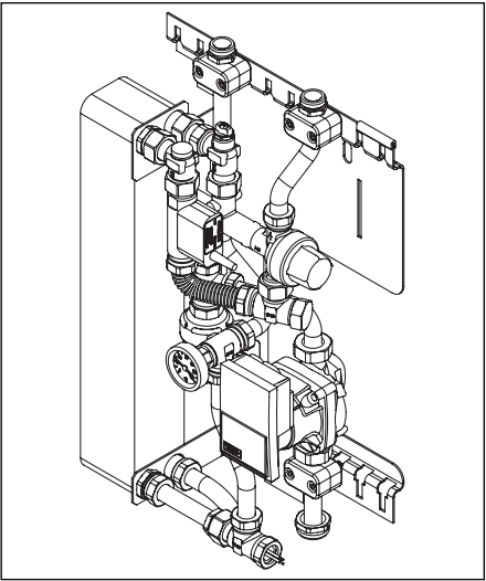
Illustr. 24 Overall view "Regumaq XH"
