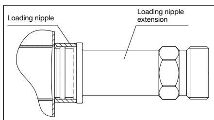
Illustr. 5 Mounted extensions for loading nipples
