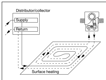
Installation sketch
