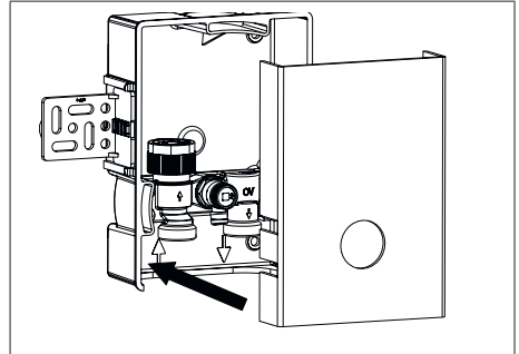
Illust. 8: Fitting of the protection cover
