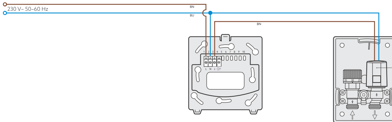
ClimaCon F 210 230 V 1155021
