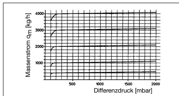
DN 40
