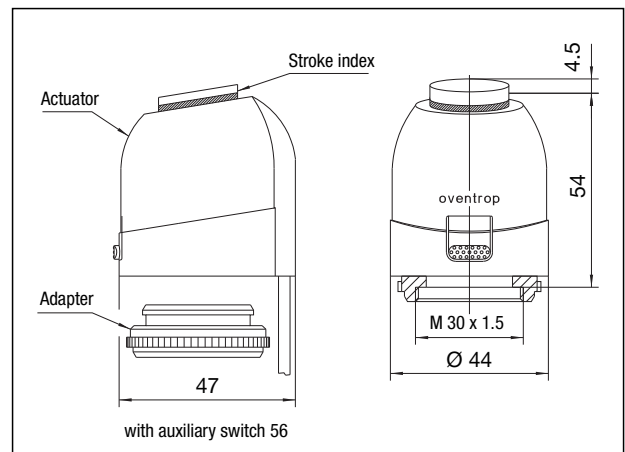
Dimensions actuators with connection thread M 30 x 1.5
