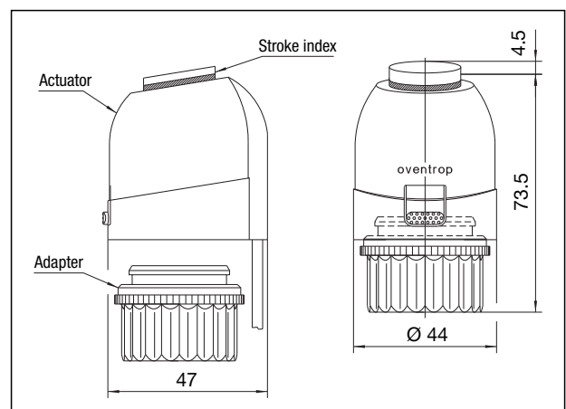
Dimensions actuators with squeeze connection
