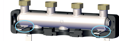
Fig. 6: Fastening of the distributor to the wall brackets
