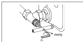
Illustr. 3 Isolation of the radiator lockshield valve
