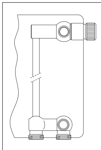
Radiator with integrated distributor G \frac{3}{4} male thread, distance between pipe centres 50 mm
