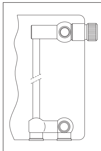
Radiator with integrated distributor G \frac{1}{2} female thread, distance between pipe centres 50 mm
