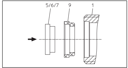
Installation of the cold water throttling disc
