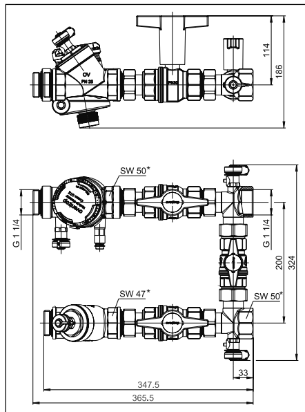
Illustr. 4.1 Dimensions "Flypass set", DN 32
