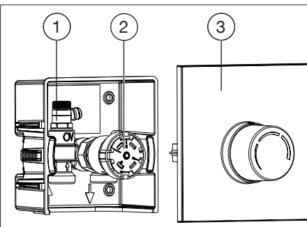
Illustr. 1: Construction “Unibox RTL vario”
