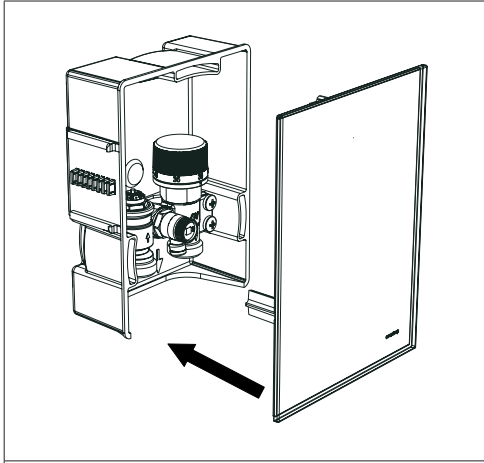
Illustr. 10: Fitting of the cover
