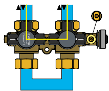
Bypass operation
