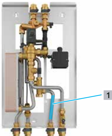
Abb. 12: Station erden
