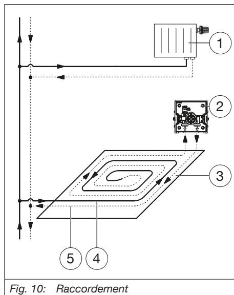
Fig. 10: Raccordement
