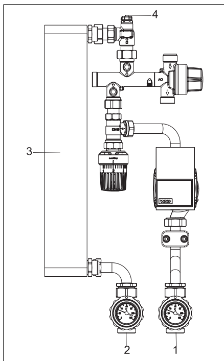
Illustr. 6.1 Bleeding "Regumaq XH"
