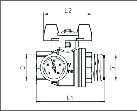
Illustr. 6: Dimensions of the ball valve
