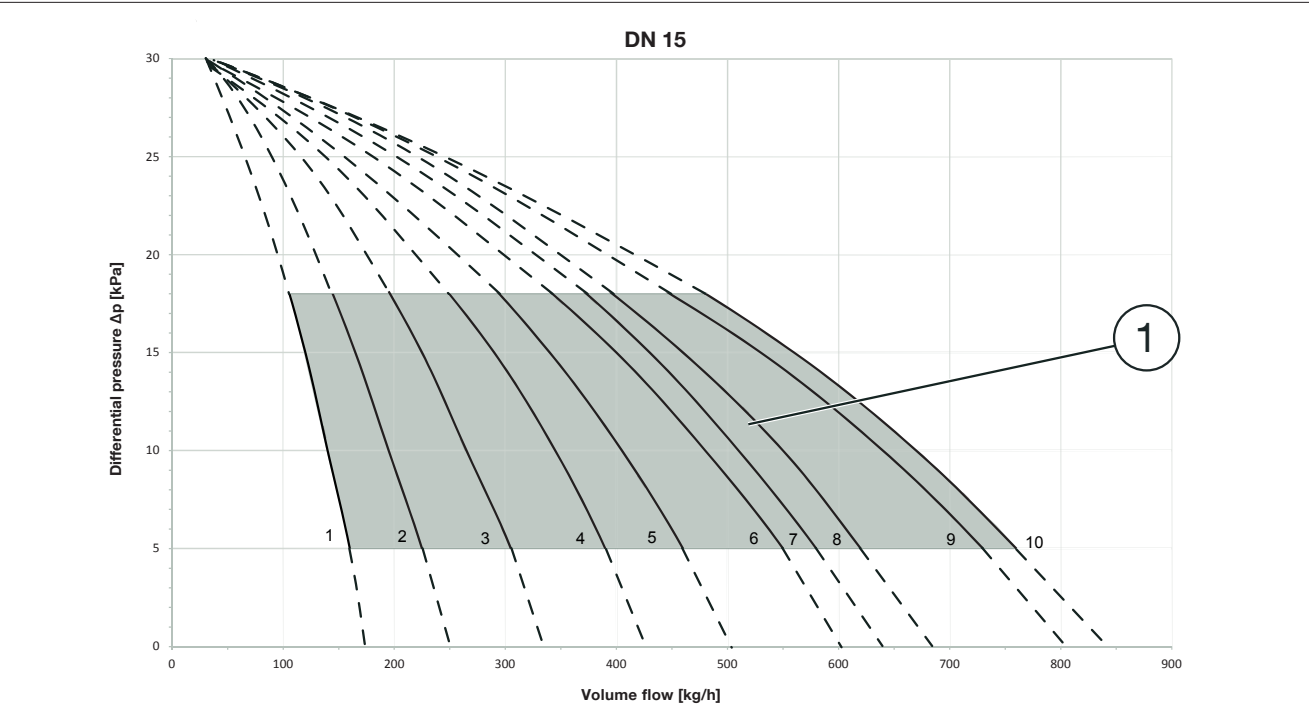
Illust. 8: Handwheel settings characteristic lines DN 15
