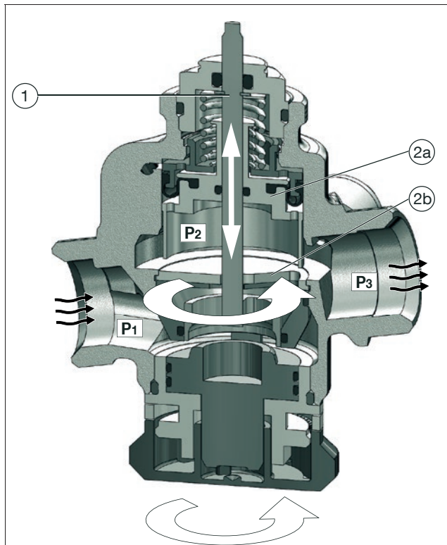
Illust. 2: "Cocon QDP" - Sectional view
