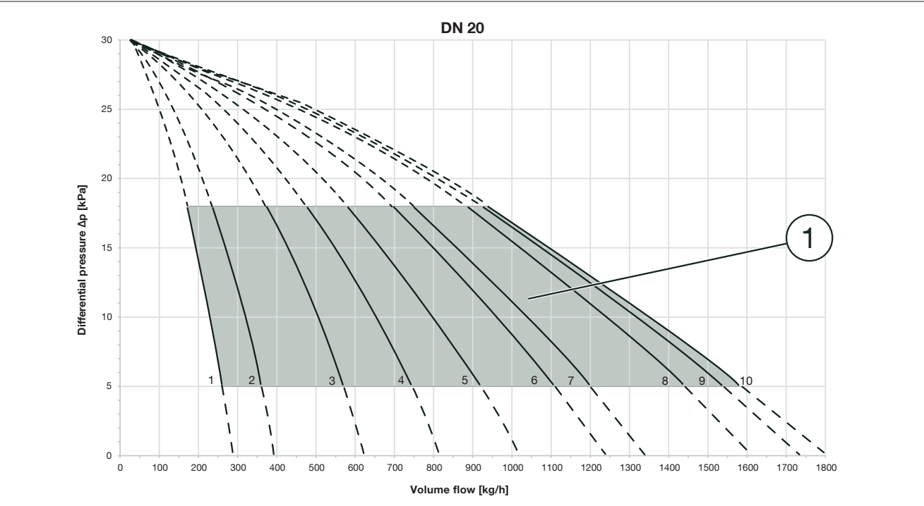
Illust. 9: Handwheel settings characteristic lines DN 20
