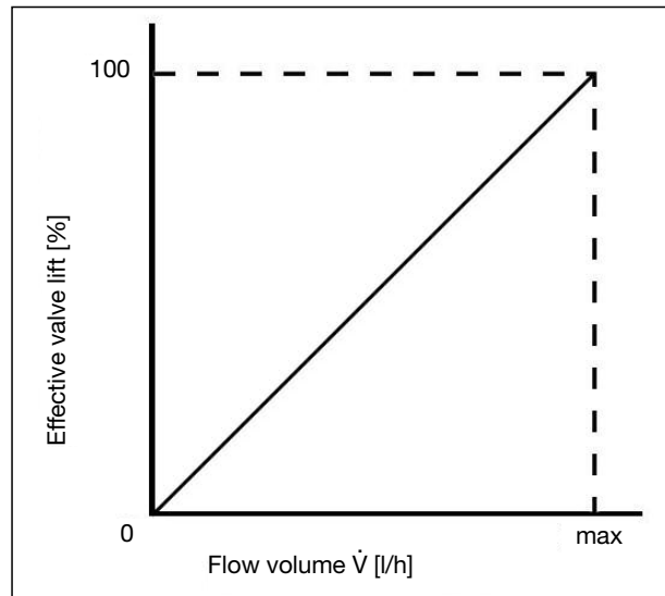
Illus. 9 Characteristic line of the valve “Cocon QFC/QGC”
