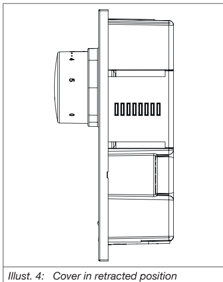
Illust. 4: Cover in retracted position
