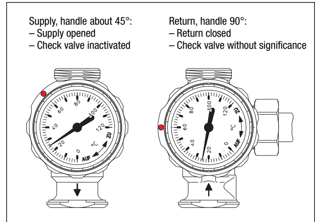
Illustr. 15: Position of the ball valves
