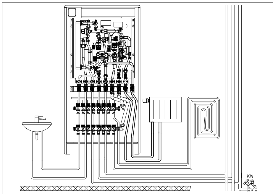
Illustr. 8.5 System illustration
