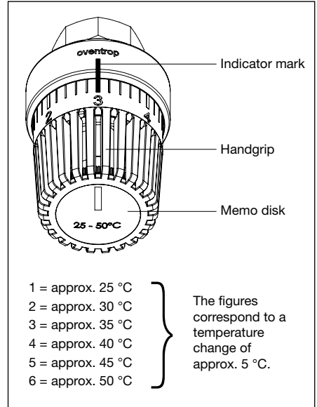
Illustr. 8.4 Setting flow temperature heating circuit
