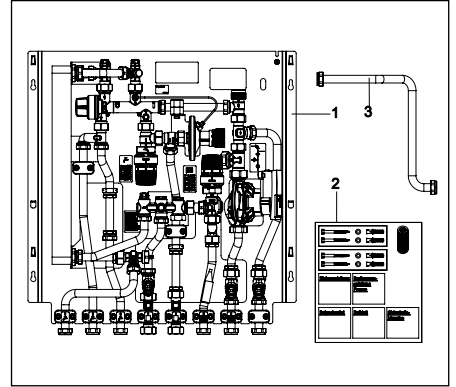
Fig. 3.1 Fourniture
