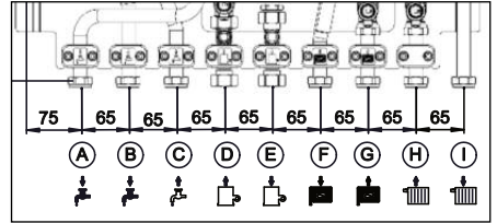
Illustr. 4.3 Connection sizes
