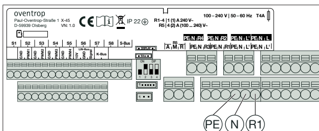
Illust. 12: Electrical connection of the circulation set
