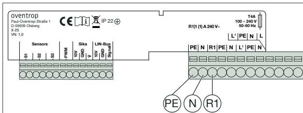
Illust. 11: Electrical connection of the circulation set
