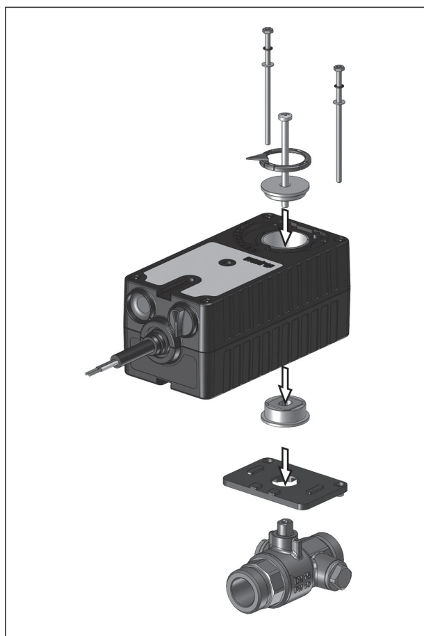
Assembly electromotive actuator and "Optibal TW"
