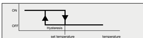
Fig. 2: ON/OFF regulation
