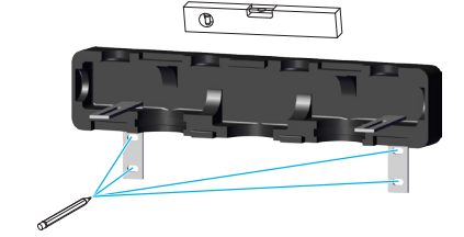
Fig. 5: Marking the drill holes
