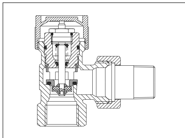
Angle pattern valve
