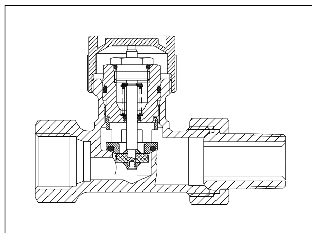
Straight pattern valve
