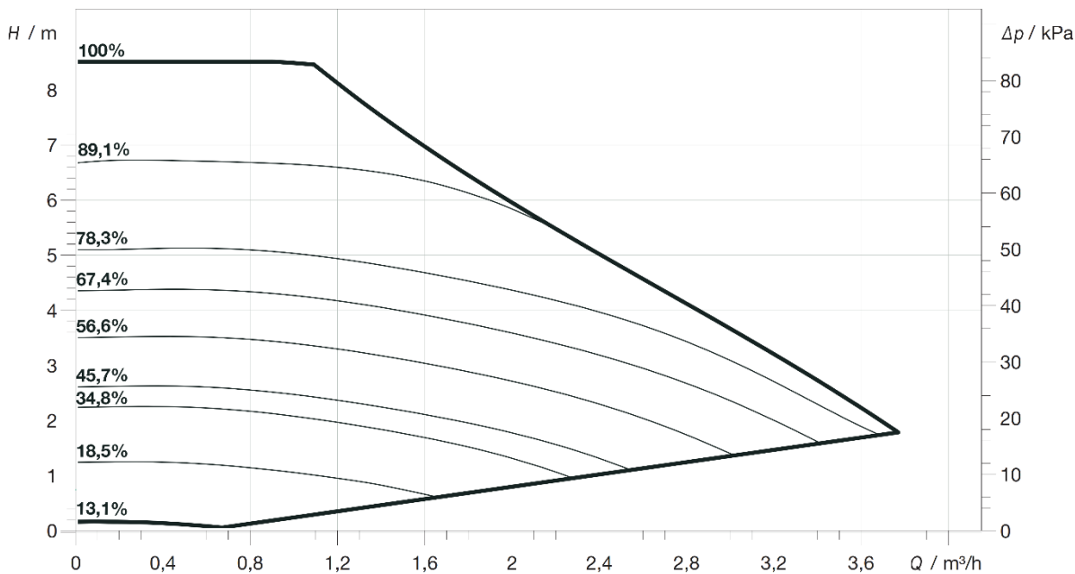
Characteristic line Wilo Para 15-130/8-75/LIN-9
