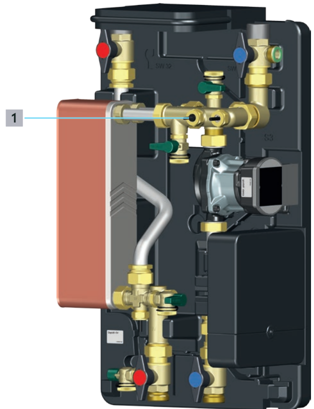
Fig. 1: Position in the Regumaq X-25 or Regumaq X-45 fresh water station
