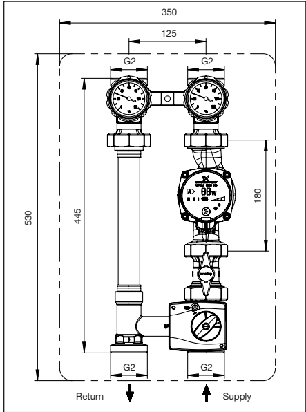
Pump group "Regumat M3-180"
