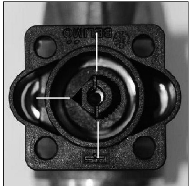
Illustr. 2: The stem of the ball valve is now aligned in the open position.
