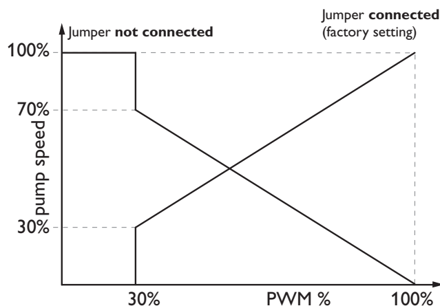
Jumper slot for the inversion of the PWM signal
