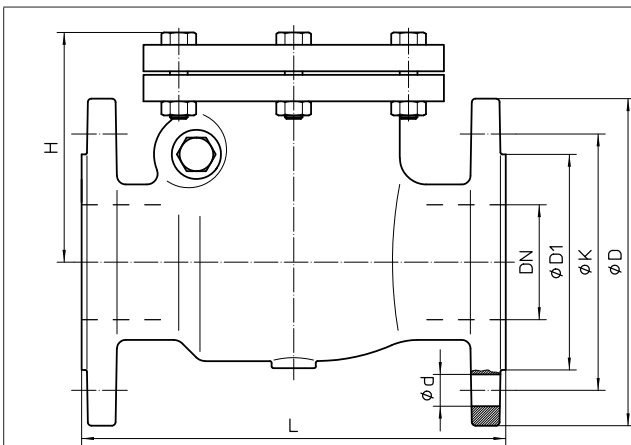
Illust. 2: Dimensions
