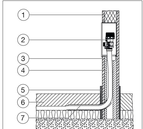
Illustr. 6: Installation cross section
