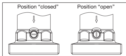
Illustr. 6.1 Check valve
