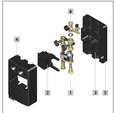
Illust. 6.6 Exploded view
