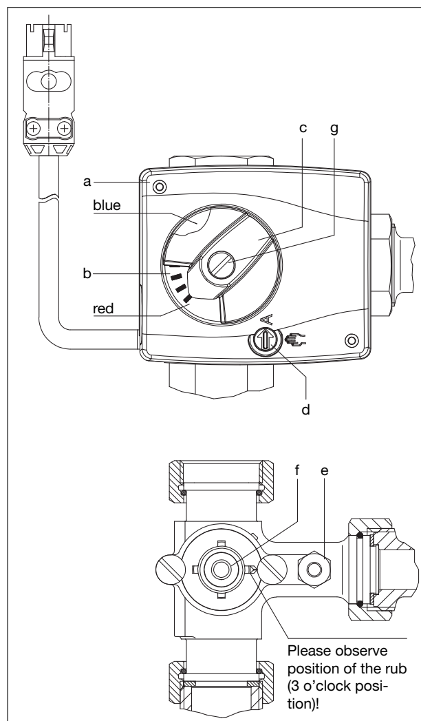
Installation actuator
