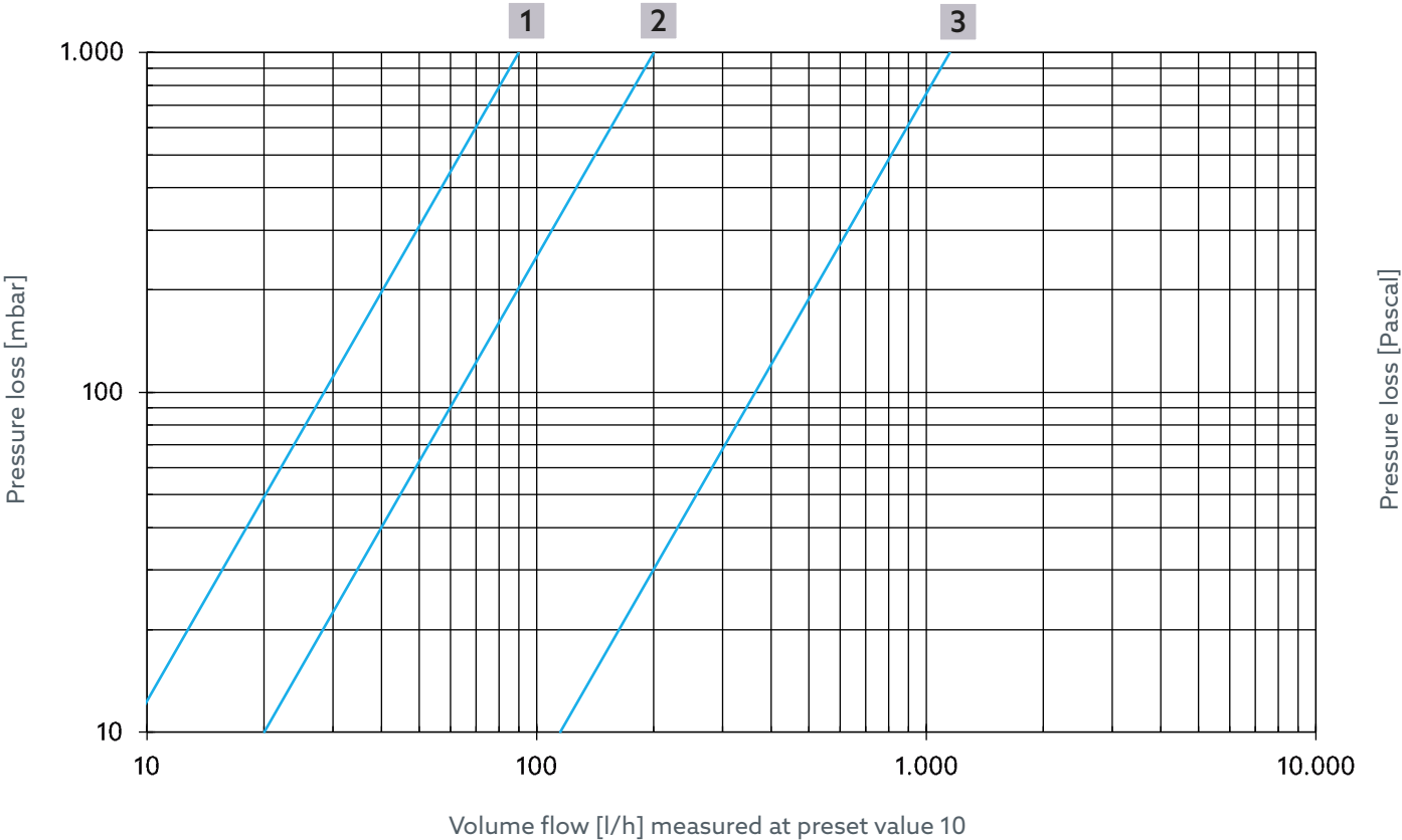
Fig. 17: Volume flow - Thermal control for item no. 4202504, 4202604, 4202704, 4202804
