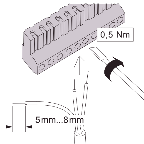
Fig. 20: Cabling of the connector plug
