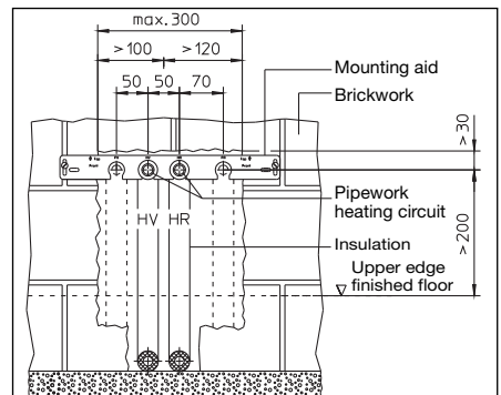
Illustr. 7 Wall view, heating circuit connection
