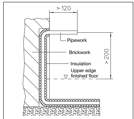
Illustr. 6 Illustrated section, heating circuit connection
