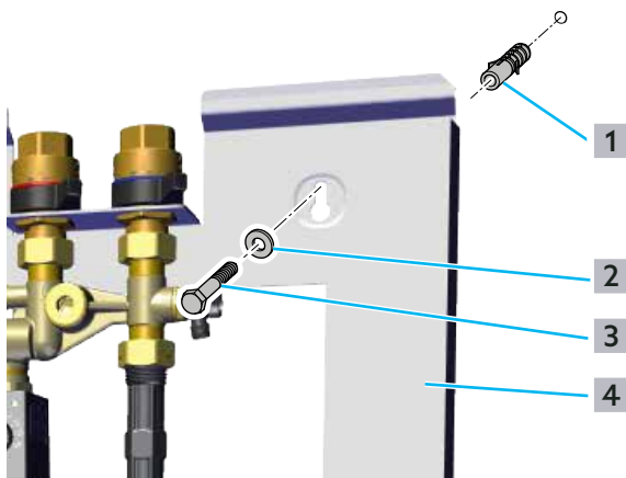
Abb. 10: Station an Wand montieren
