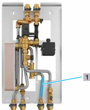
Abb. 12: Station erden
