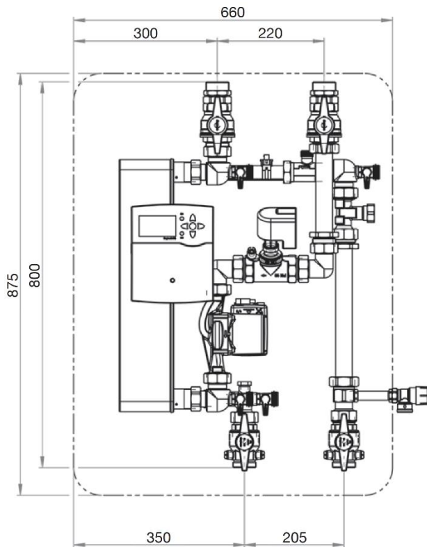
Abmessungen Regumaq X-70 (Front)
