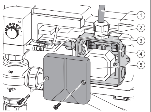
Illustr. 1: Construction
