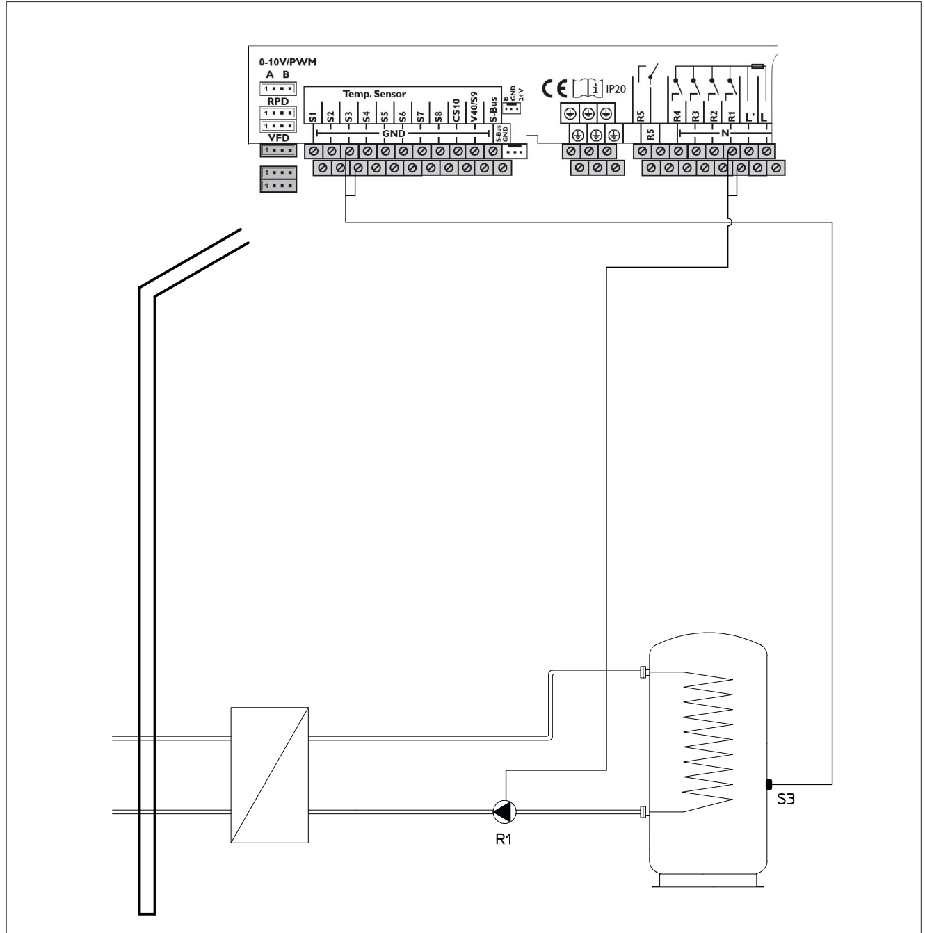
Illust. 51: Scheme 7, indirect hot potable water preparation
