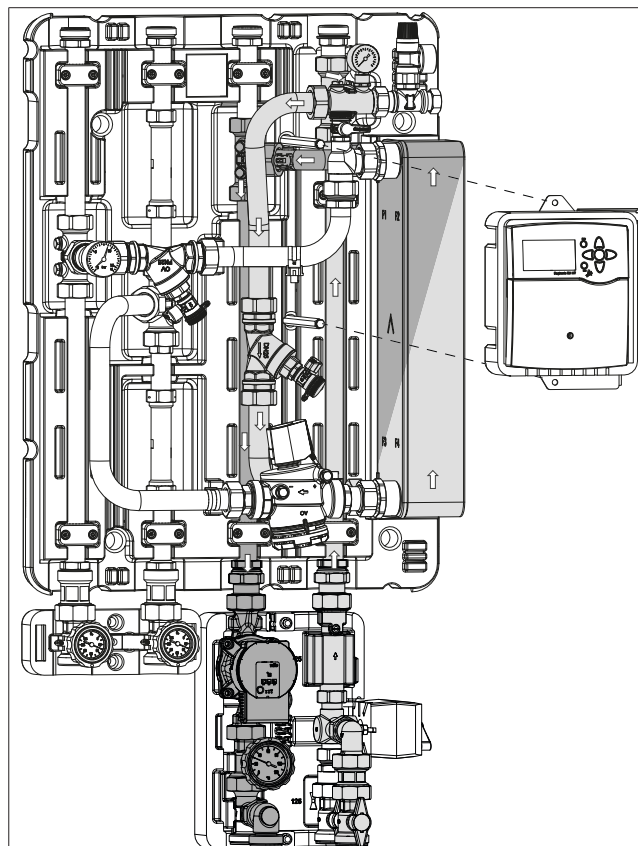
Illust. 22: Secondary side - Connection of the storage cylinder circuit Regudis H-HT / Regudis H-MT (bottom connection)
