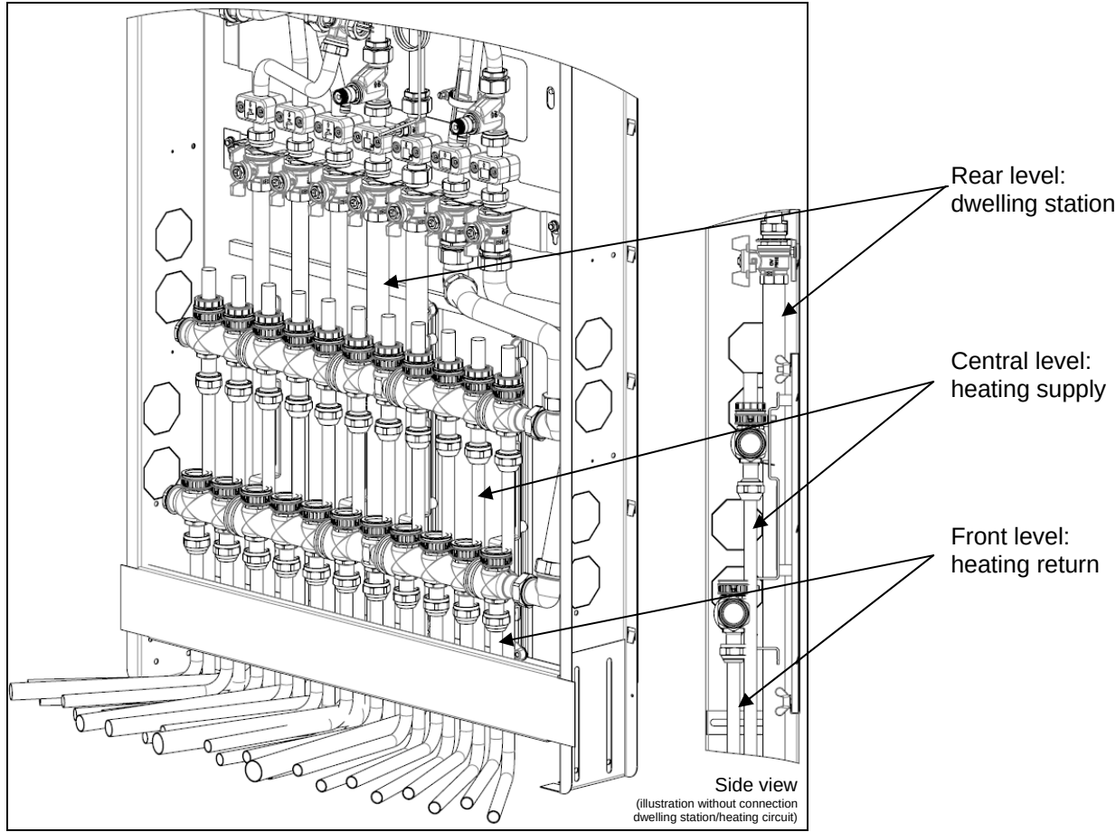
Piping example:
