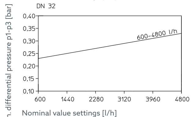
Fig. 13: Minimum differential pressures
