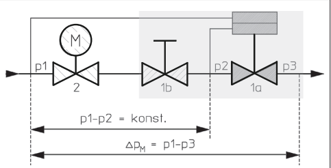
Illust. 3: Function of “Cocon QTZ”, PN 25
