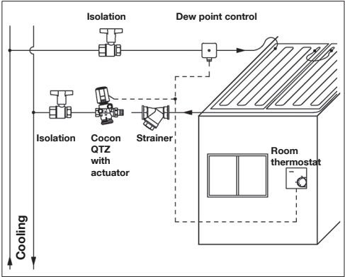
Illust. 6: Installation example 1: Two pipe system
