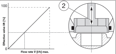
Illust. 5: Linear characteristic line of the regulating unit
