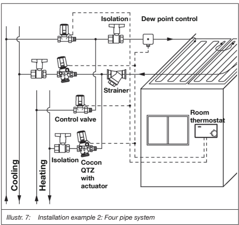
Illust. 7: Installation example 2: Four pipe system
