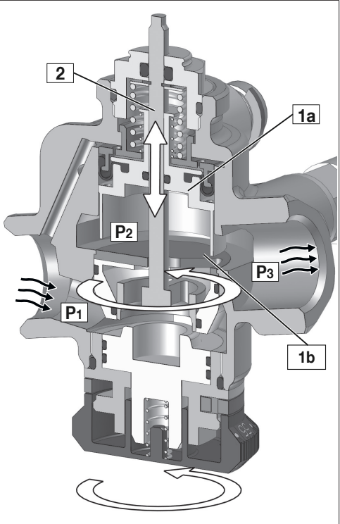
Illust. 2: Illustrated section “Cocon QTZ”
