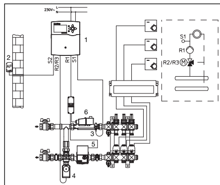
1 = "Regtronic RH-B" heating circuit controller S1 = Flow sensor variable temperature circuit (3) S2 = Outdoor sensor (2) R2/R3 = Actuator mixing valve (4) R1 = Pump variable temperature circuit (5) 6 = "Regufloor HW" ("Regtronic RH-B" included)
